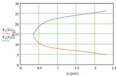
Calcite: L/A=2.5 (350-2300nm)
