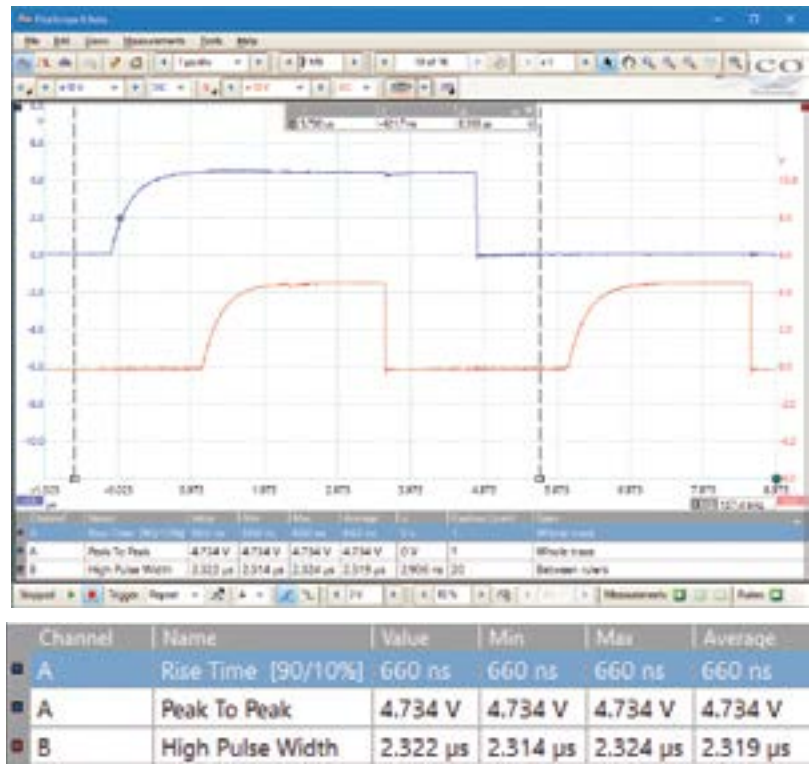
Scope mode
