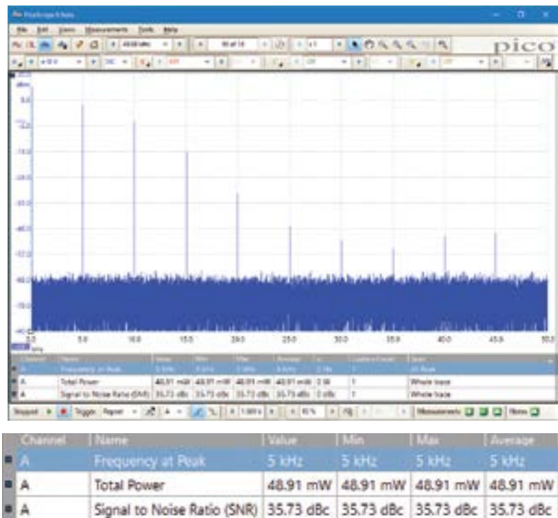
Spectrum mode
