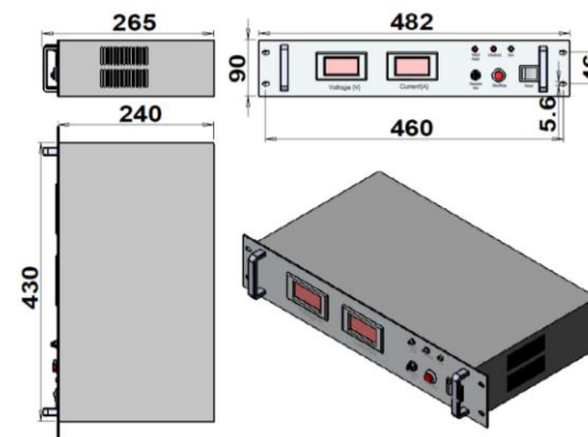
PSU-HPL-QS(12U)-3 482(L) × 265(W) × 90(H)mm 3 , 13kg
