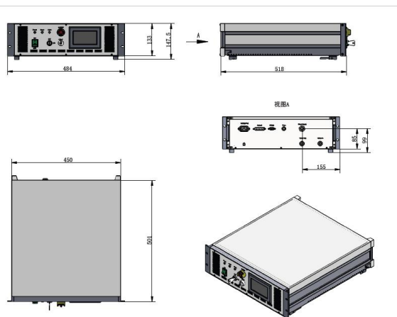
518 (L)×450(W)×147.5(H)mm 3 ,
