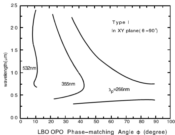
Figure 4. Type I OPO tuning curves of LBO
