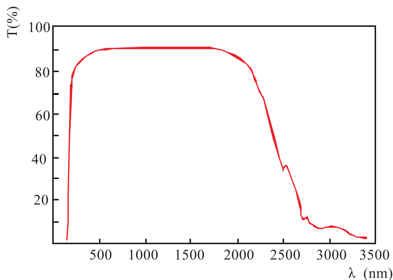
Figure 1. Transparency curve of LBO
